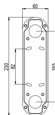
WALL PLATE
